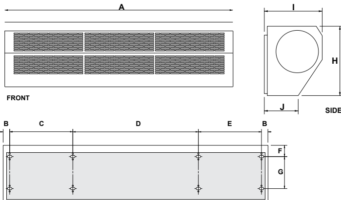
BACK (mounting plate is shaded portion)
